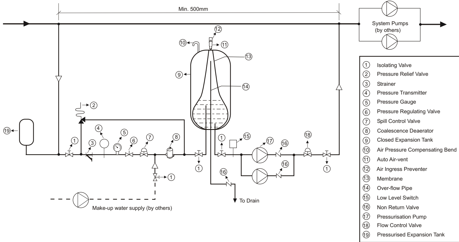
Schematic drawing of Hydronic Pressurisation Systems
